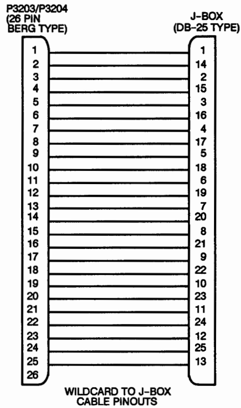
Figure 1. Wildcard to Junction Box Cabling Detail
